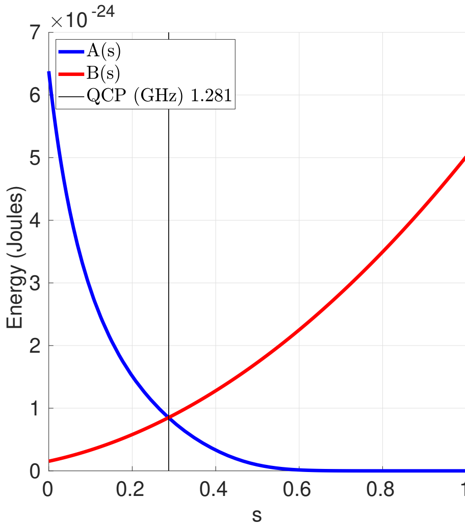
Figure 2.2: Standard annealing schedule for the QPU, showing energy changes as a function of scaled time.
